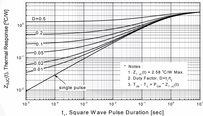
Figure 11-2. Transient Thermal Response Curve for FDPF55N06
