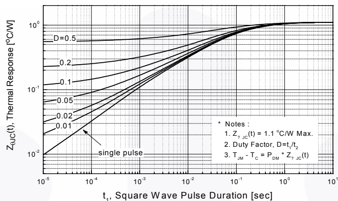
Figure 11-2. Transient Thermal Response Curve for FDPF55N06
